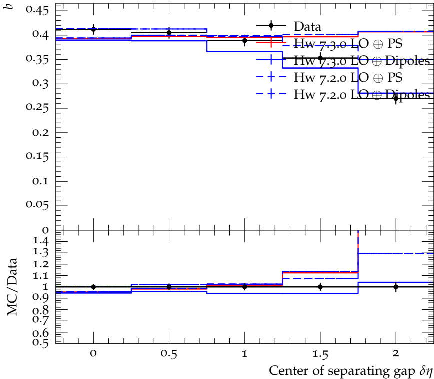
Forward-backward correlation b vs. gap center \sqrt{s} = 546 GeV
