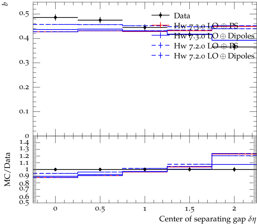
Forward-backward correlation b vs. gap center \sqrt{s} = 900 GeV
