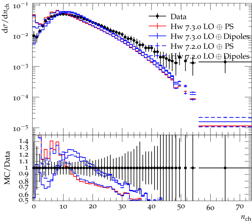
Charged multiplicity at \sqrt{s} = 200 GeV, |\eta| < 3.0
