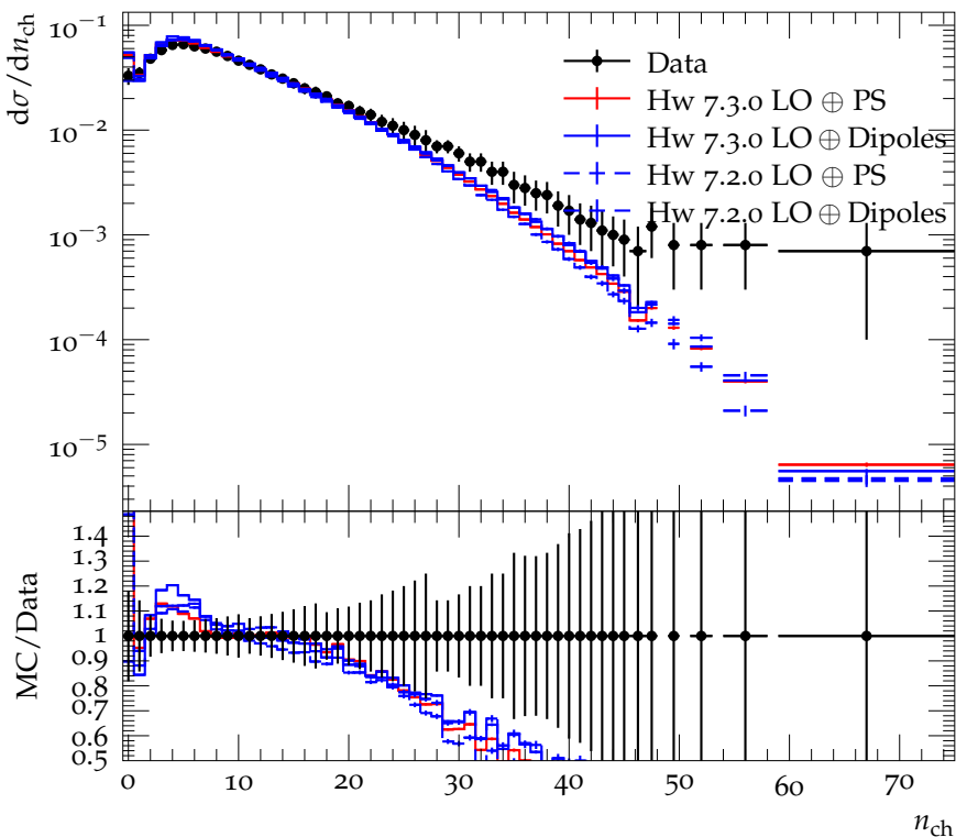
Charged multiplicity at \sqrt{s} = 900 GeV, |\eta| < 1.5
