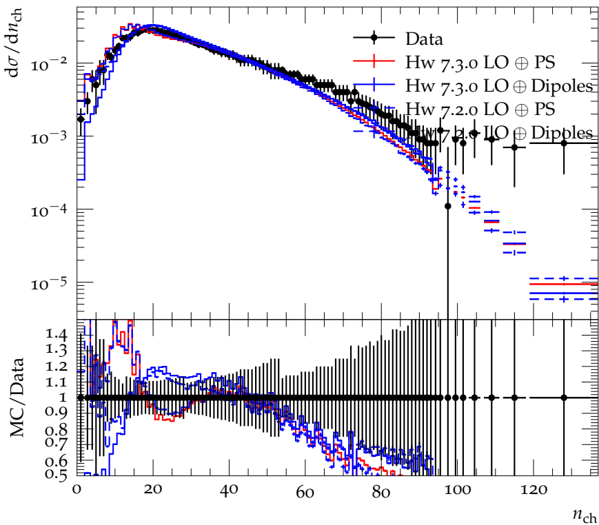
Charged multiplicity at \sqrt{s} = 900 GeV, |\eta| < 5.0
