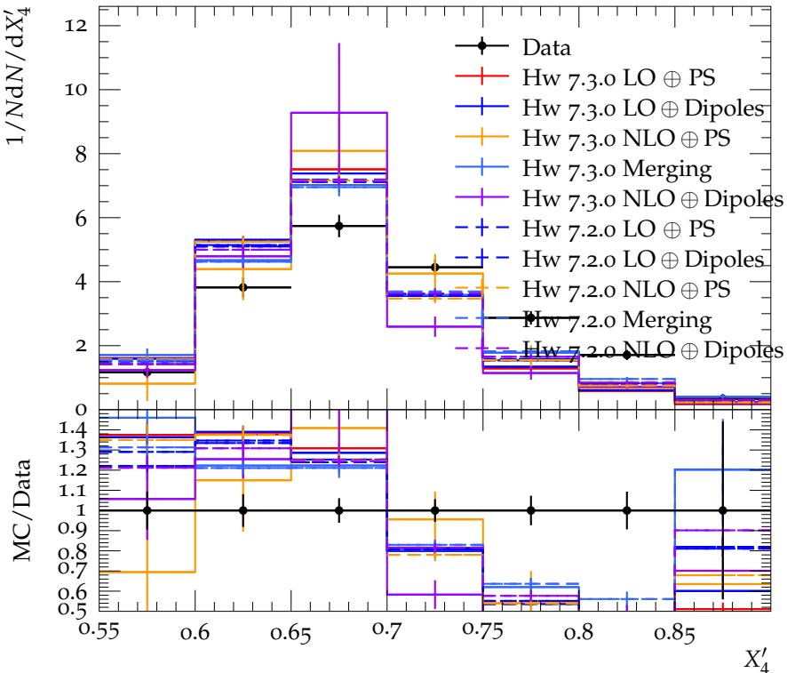
Dalitz distribution in inclusive 4-jet events
