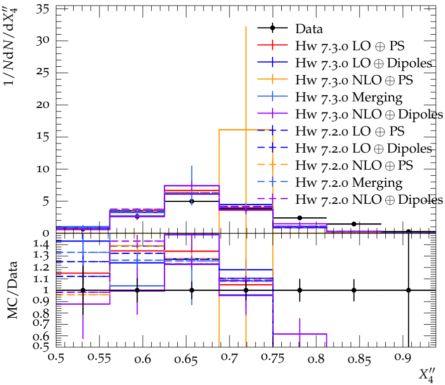
Dalitz distribution in inclusive 5-jet events
