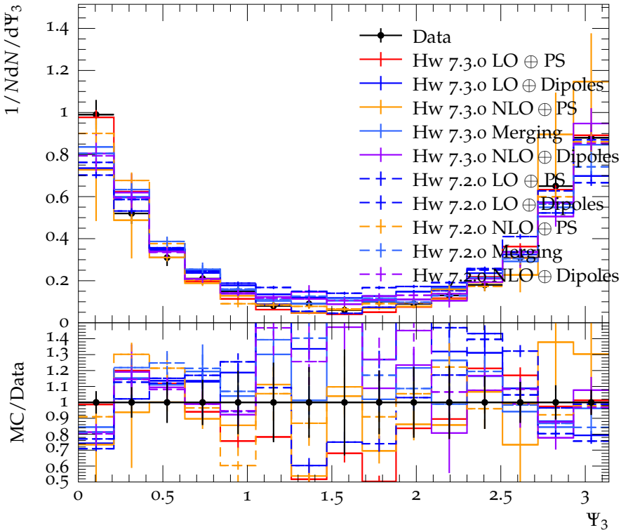
Angular distribution in inclusive 3-jet events
