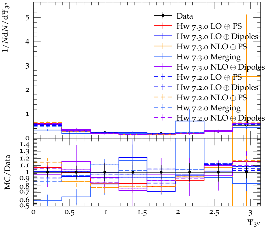
Angular distribution in inclusive 5-jet events
