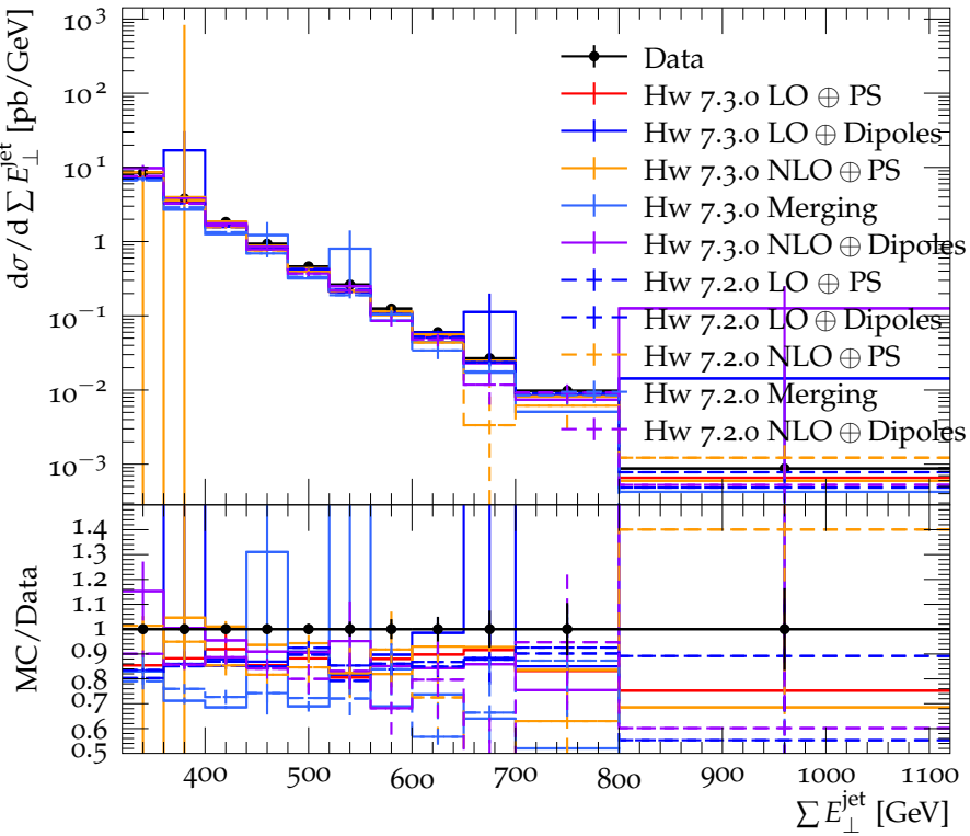
E_{\perp} sum for jets with E_{\perp} > 100 GeV
