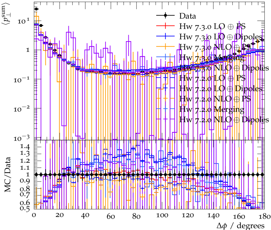
\langle p_{\perp}^{\text{sum}} \rangle vs. \Delta\phi from leading jet ( p_{\perp}^{\text{lead}} > 30 GeV)
