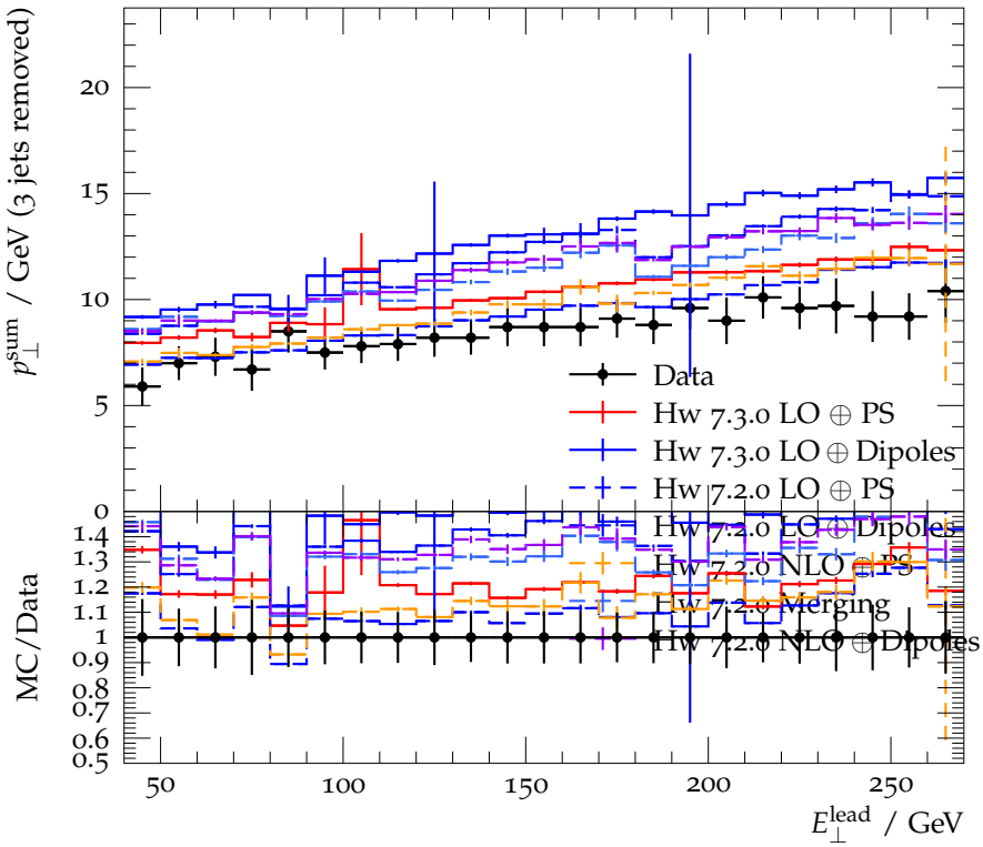
Swiss Cheese p_{\perp}^{\text{sum}} vs. E_{\perp}^{\text{lead}} (3 jets removed) at \sqrt{s} = 1800 GeV
