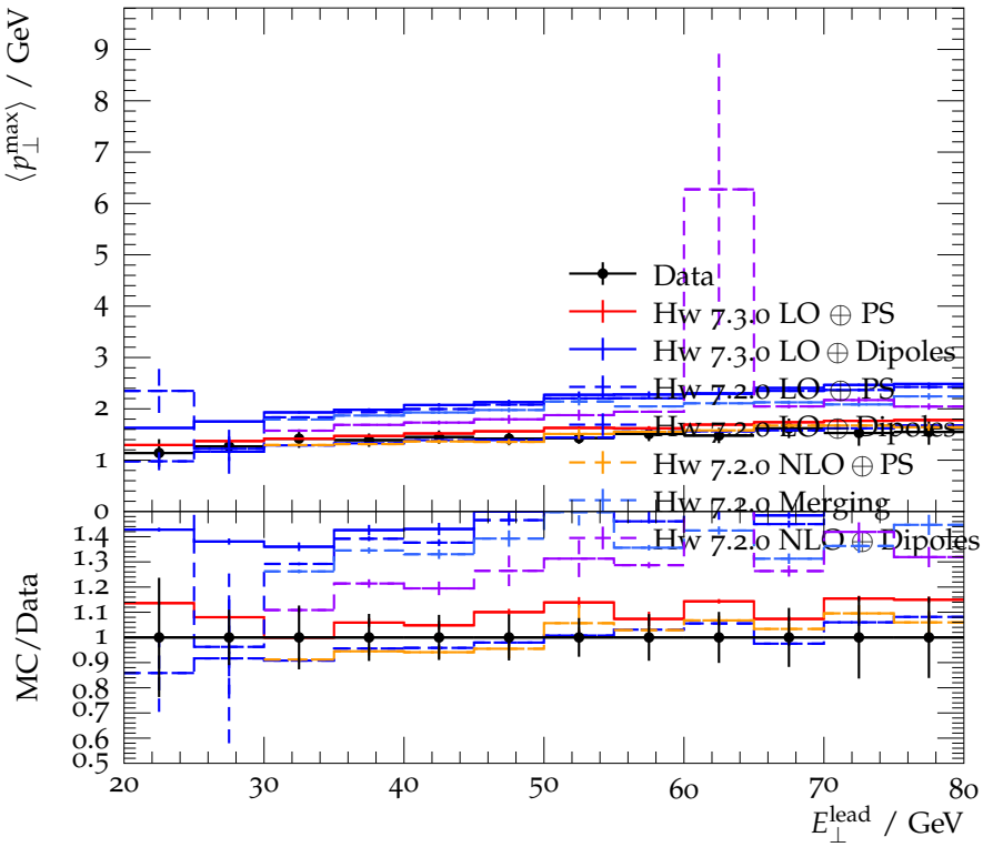
Transverse cone \langle p_{\perp}^{\max} \rangle vs. E_{\perp}^{\text{lead}} at \sqrt{s} = 630 GeV
