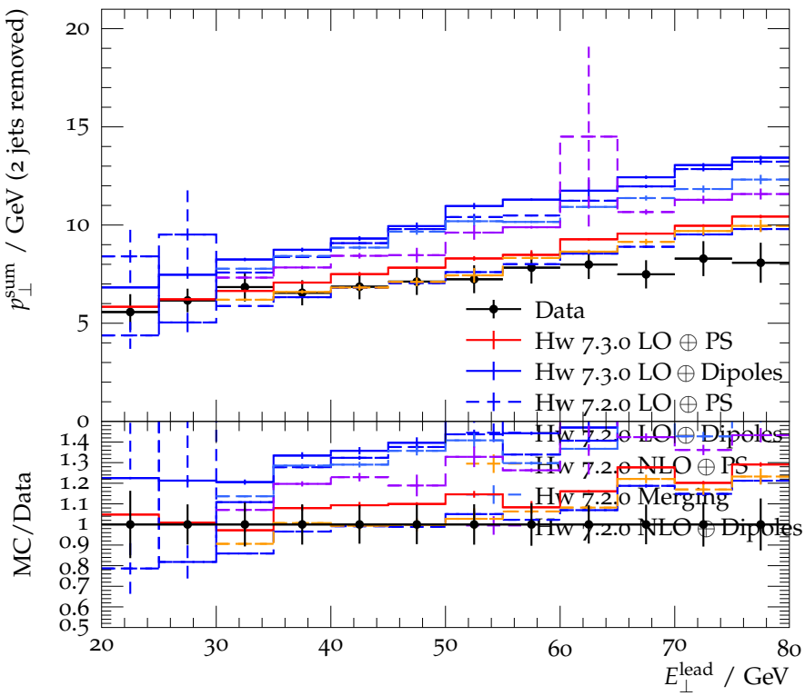
Swiss Cheese p_{\perp}^{\text{sum}} vs. E_{\perp}^{\text{lead}} (2 jets removed) at \sqrt{s} = 630 GeV
