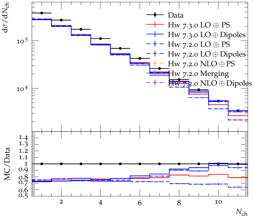
Min bias track multiplicity distribution at \sqrt{s} = 630 GeV
