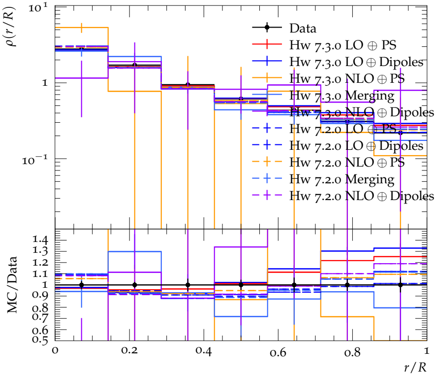
Differential jet shape \rho , 55 \text{ GeV}/c < p_{\perp}^{\text{jet}} < 63 \text{ GeV}/c
