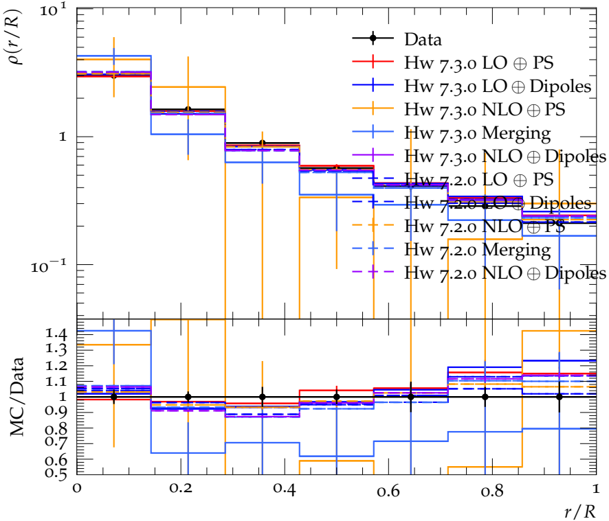
Differential jet shape \rho , 63 \text{ GeV}/c < p_{\perp}^{\text{jet}} < 73 \text{ GeV}/c
