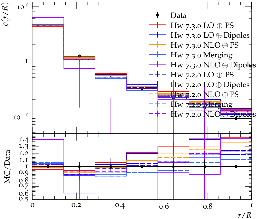
Differential jet shape \rho , 186 \text{ GeV}/c < p_{\perp}^{\text{jet}} < 208 \text{ GeV}/c
