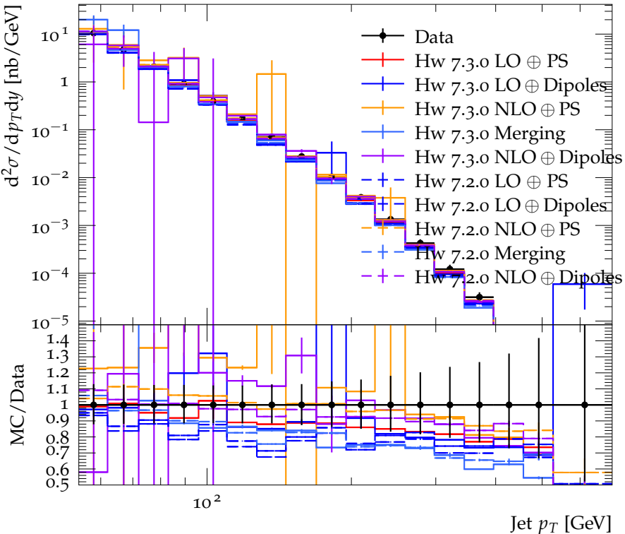
Inclusive jet cross-section vs p_T for 0.1 < |\eta| < 0.7, D = 0.5
