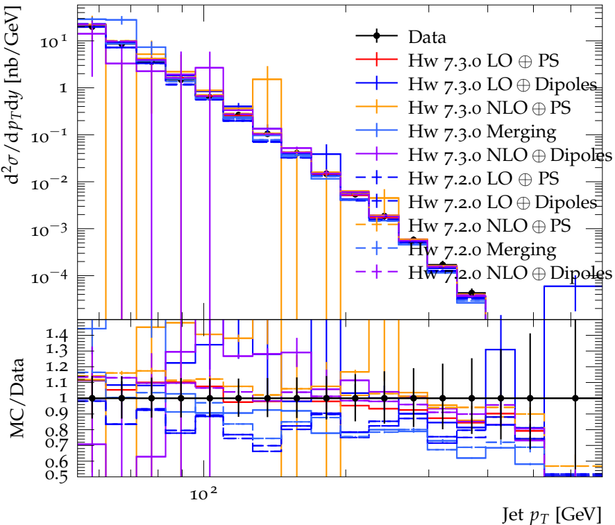
Inclusive jet cross-section vs p_T for 0.1 < |\eta| < 0.7, D = 1.0
