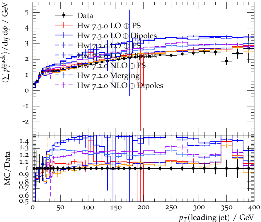
TransMAX region charged \Sigma p_{\perp} density
