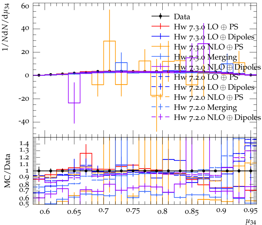
Scaled invariant mass of jet pair
