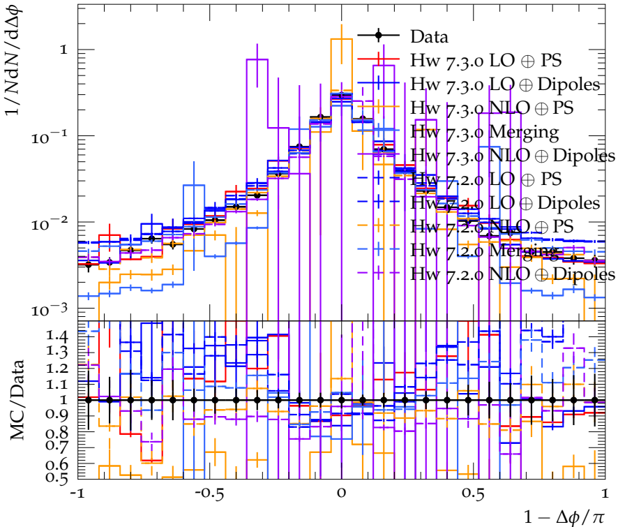
Azimuthal angle difference for 2 < \Delta\eta < 4
