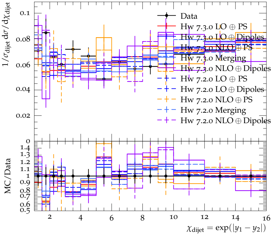
Dijet angular distribution in 0.4 < M_{jj}/\text{TeV} < 0.5
