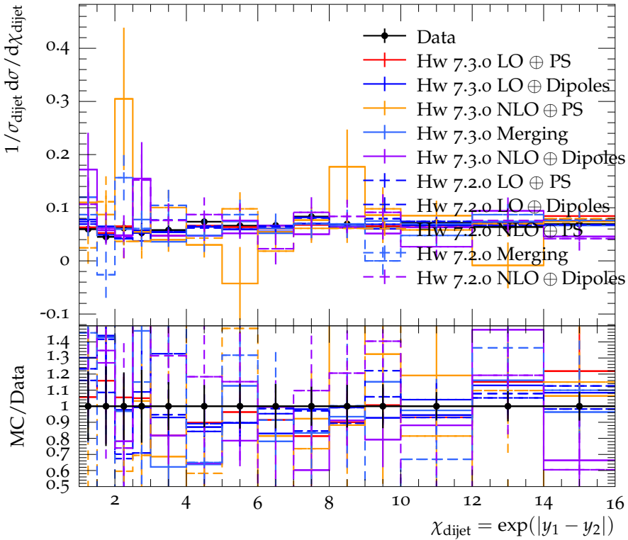
Dijet angular distribution in 0.7 < M_{jj}/\text{TeV} < 0.8
