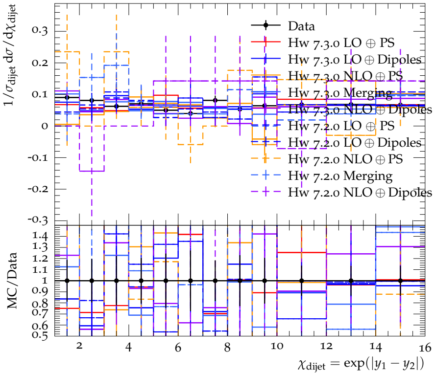
Dijet angular distribution in 0.9 < M_{jj}/\text{TeV} < 1.0
